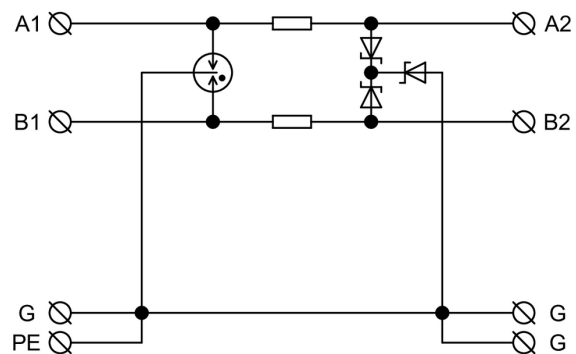
Internal diagram
